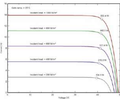
I-V-CURVE
