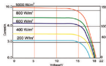
I-V-CURVE
